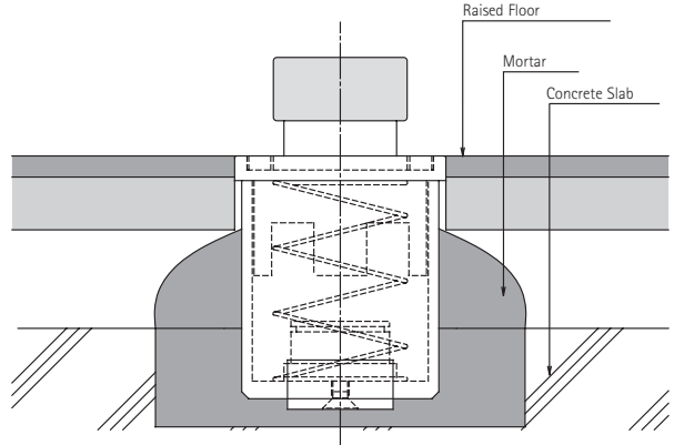
Raised Floor
